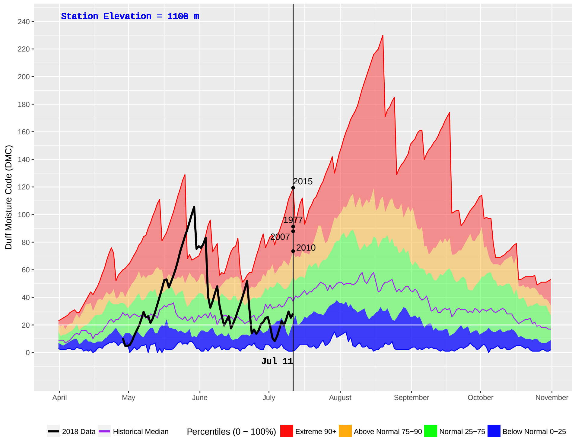
PALLISER (411) : Historical (1973–2016) and Current (2018) Noon Duff Moisture Code (DMC)
