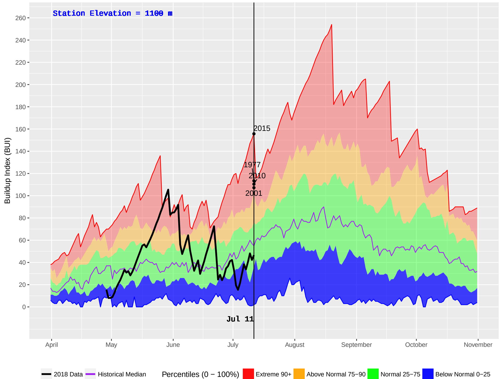
PALLISER (411) : Historical (1973–2016) and Current (2018) Noon Buildup Index (BUI)
